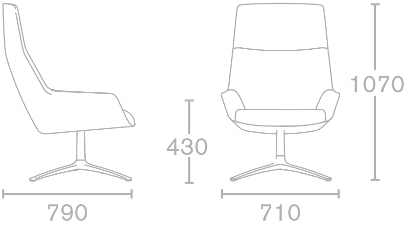
High back swivel base
